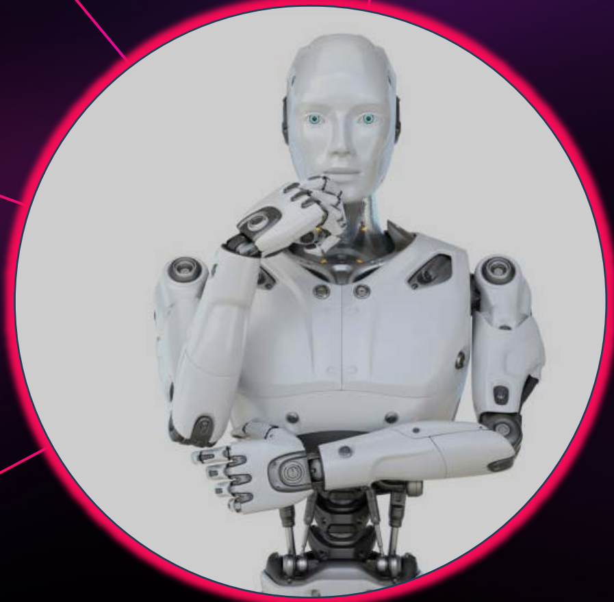
Adversarial examples
